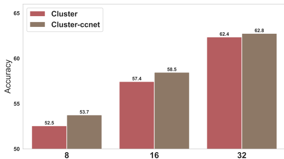
Figure 2: Changing domain of tasks from Wikipedia to CommonCrawl (ccnet) while keeping size of data, compute and model fixed. Overall average across 19 downstream tasks is shown. More diverse domain (ccnet) in training leads to improved down-stream accuracy.
